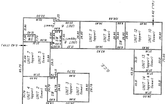
PLAN - FIRST & SECOND FLOORS Scale: 1" = 20"
